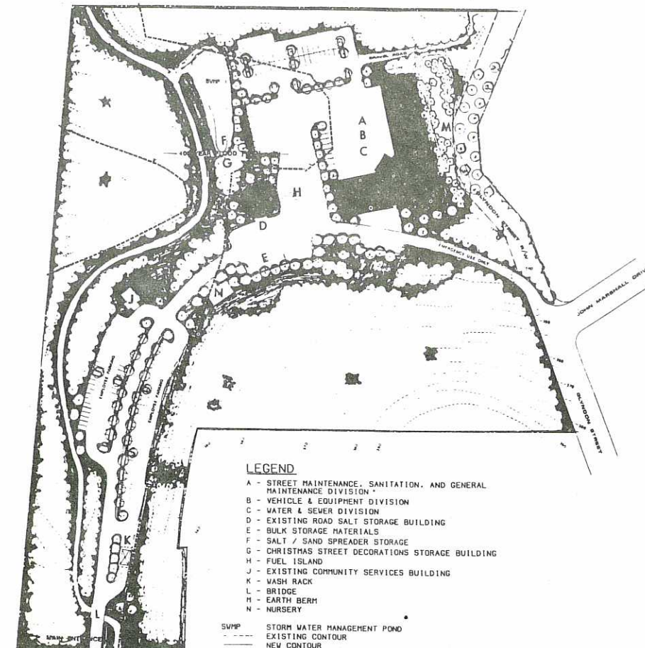
NORTHSIDE PROPERTY YARD PROPOSED MASTER PLAN
