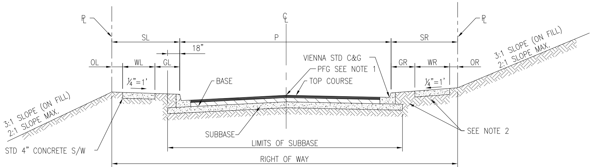
TYPICAL SECTIONS
